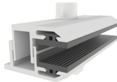
MG-TF-EC-L80 Thin Film End Clamp, 80 mm MG-TF-EC-L120 Thin Film End Clamp, 120 mm
